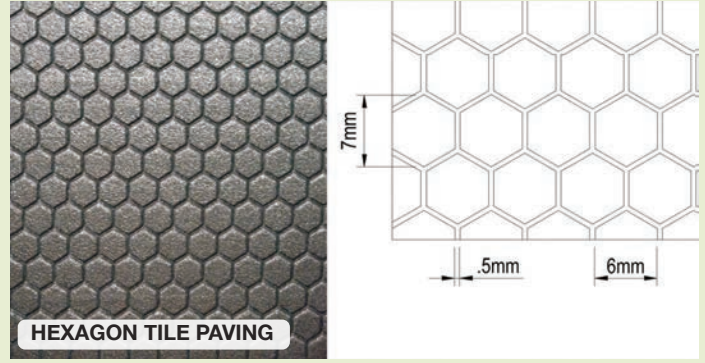
FLOORBOARDS NM015 / NM015A Small scale
