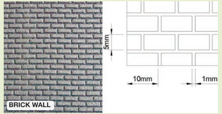
NM005 / NM005A Small scale / NM005B Double sided 10mm
