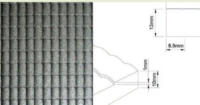
NM022 / NM022A Small scale
