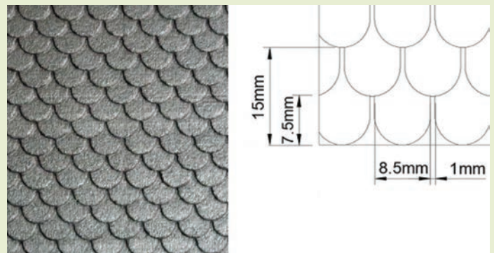
NM023 / NM023A Small scale
