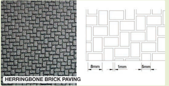
NM007 / NM007A Small scale
